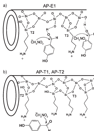
Scheme 2. Reaction mechanism to explain the enhanced efficiency of AP-E1 (a) in the Henry reaction relative to AP-T1 and AP-T2 (b). The presence of a significant number of spatially isolated silanol groups in AP-E1 leads to activation of the carbonyl group of benzaldehyde for nucleophilic attack. [11]
